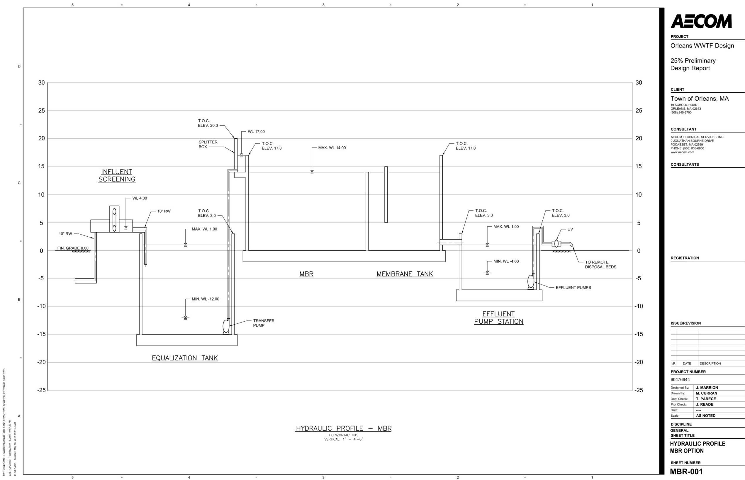
Figure 14: Hydraulic Profile – MBR Option
