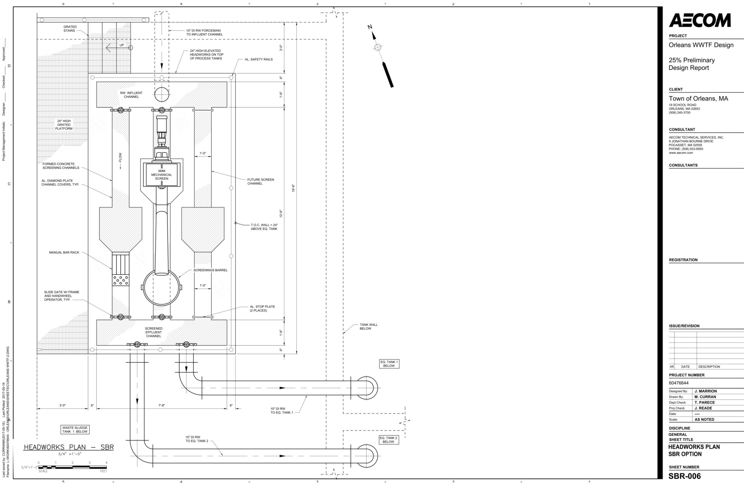
Figure 8: Headworks Layout – SBR Option
