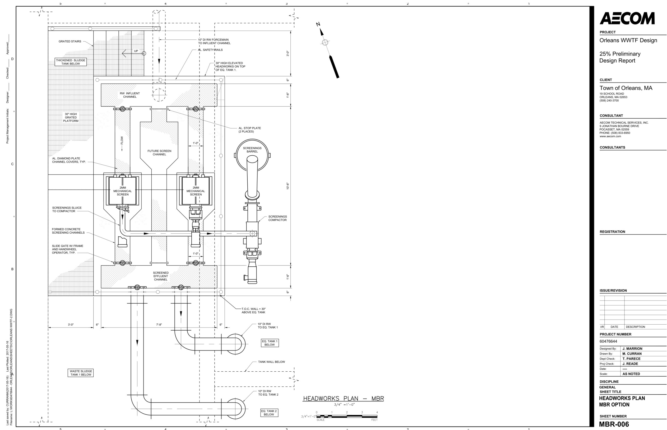
Figure 7: Headworks Layout – MBR Option
