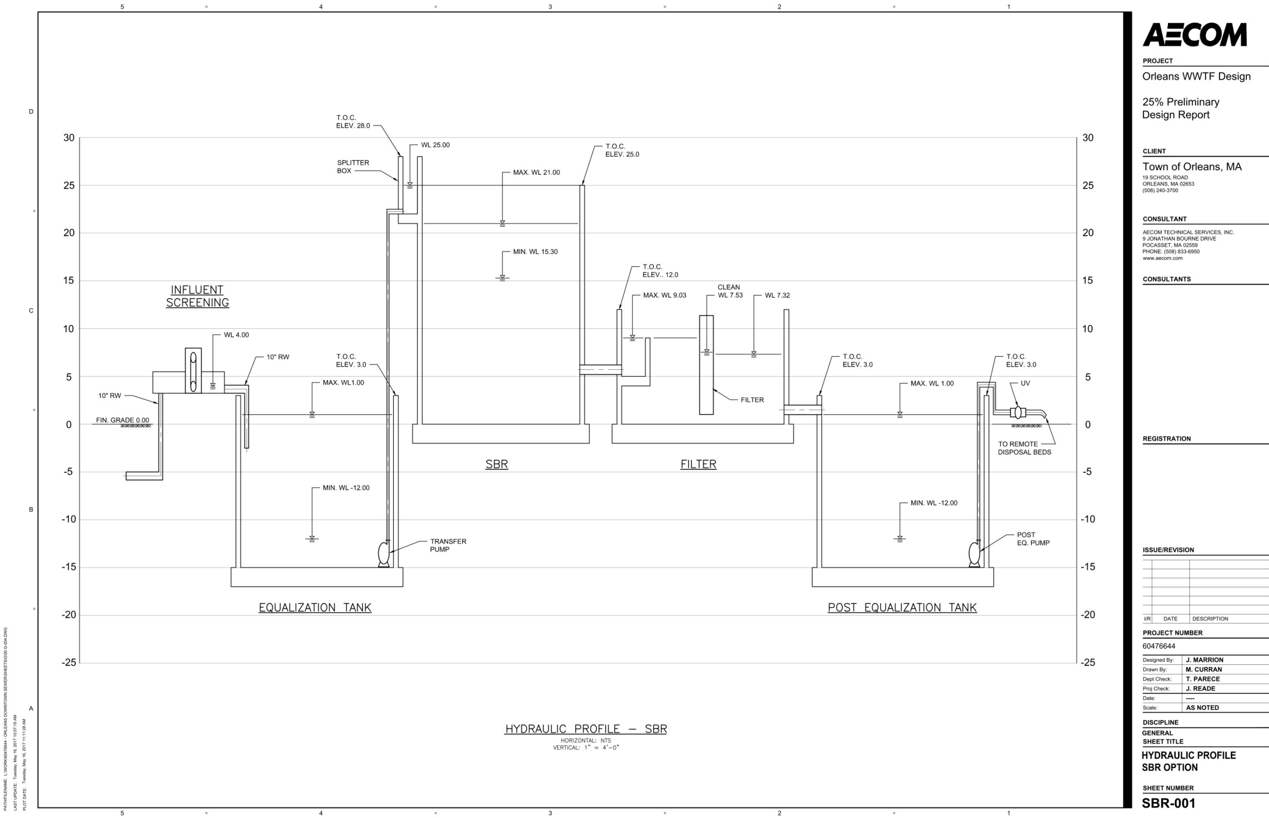
Figure 18: Hydraulic Profile – SBR Option
