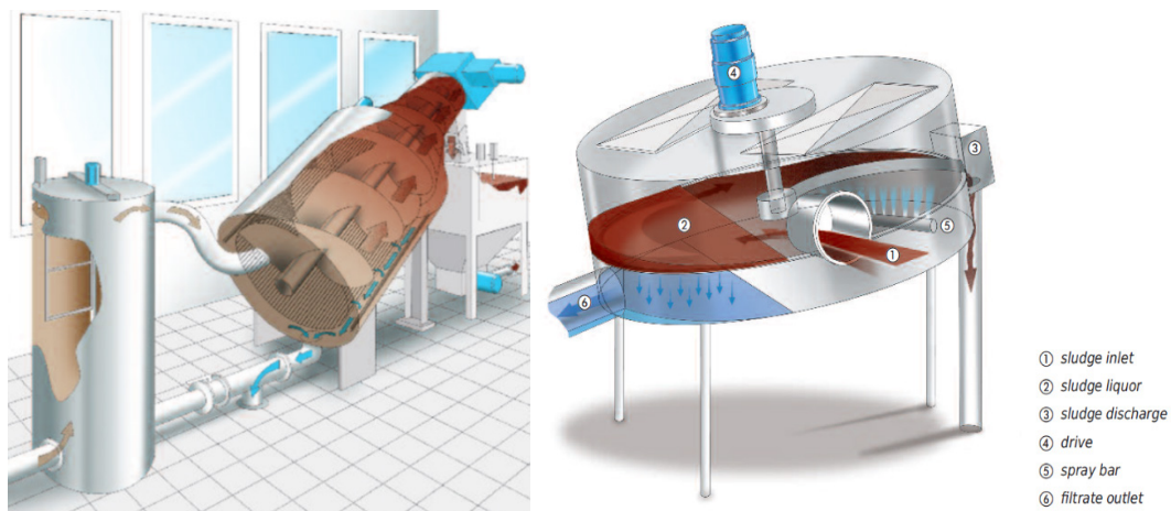
Figure 4: Example of Disk Thickener (Huber Technology, Inc.)
