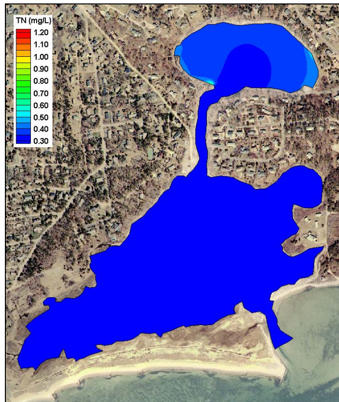
Figure VIII-3. Contour Plot of modeled total nitrogen concentrations (mg/L) in the Taylors Pond/Mill Creek system, for threshold loading conditions (0.38 mg/L in Taylors Pond).
