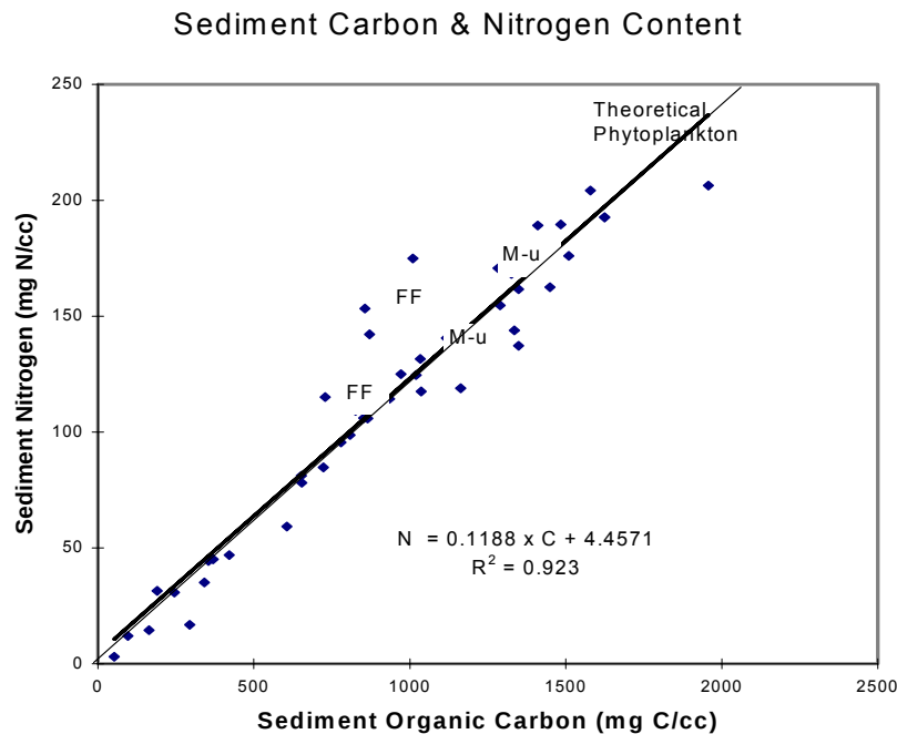
Figure IV-9 Sediment Carbon vs. Sediment Nitrogen content for core samples taken from Chatham sub-embayments
