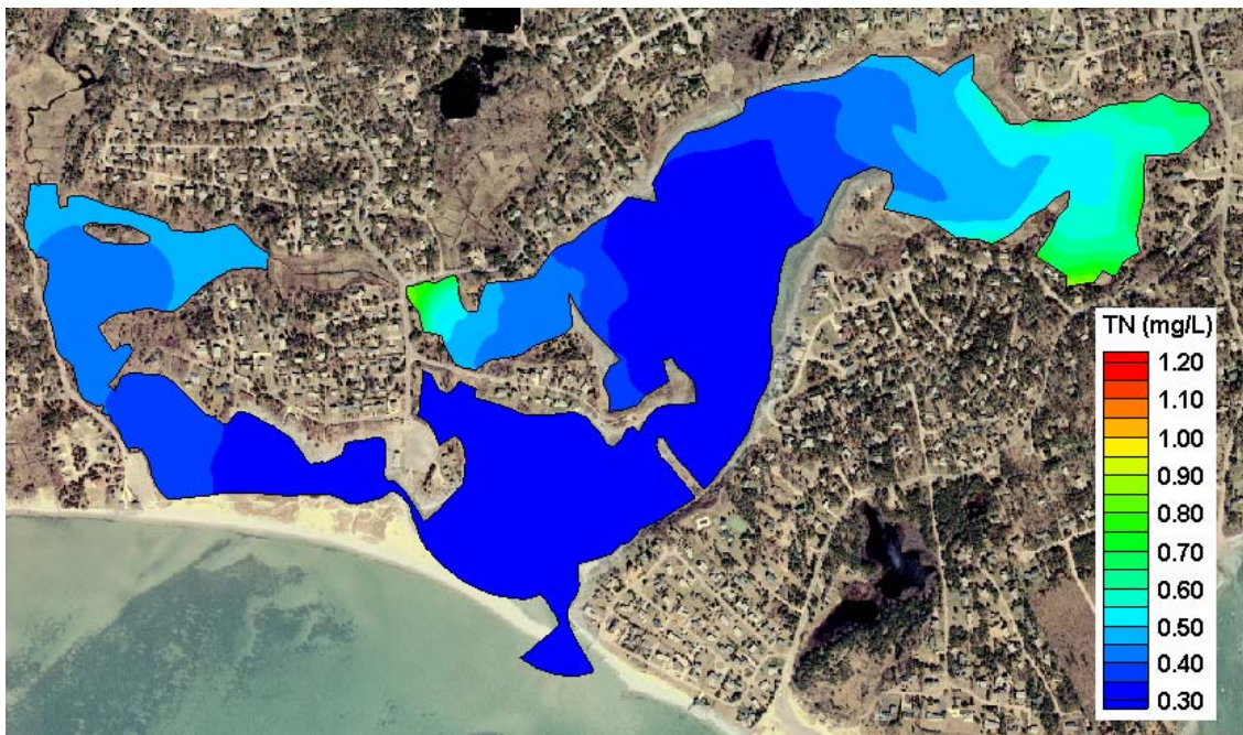
Figure VI-16. Contour Plot of modeled total nitrogen concentrations (mg/L) in the Sulphur Springs/Cockle Cove Creek system, for no anthropogenic loading conditions.
