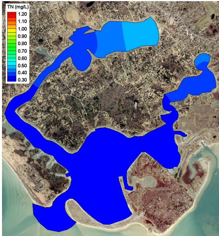
Figure VI-15. Contour Plot of modeled total nitrogen concentrations (mg/L) in the Stage Harbor system, for no anthropogenic loading conditions.
