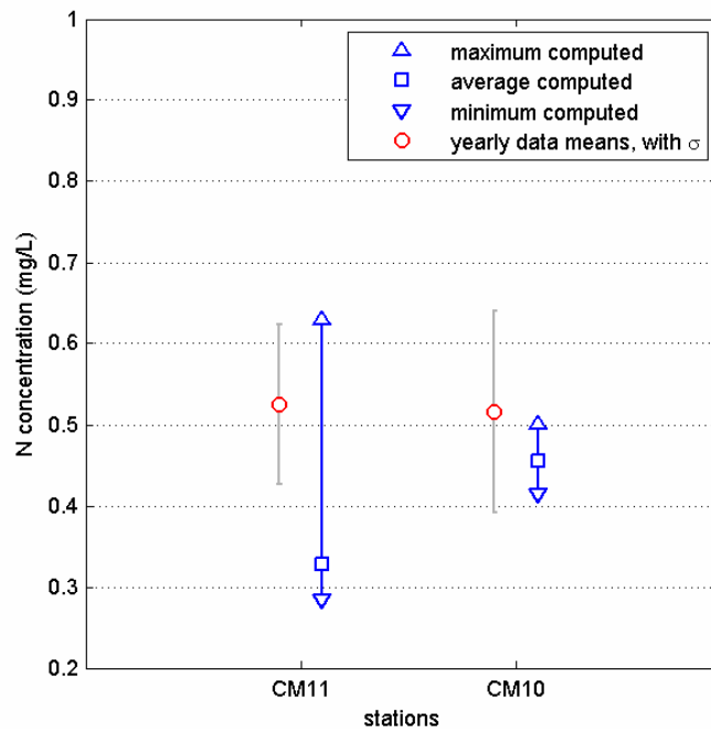
Figure VI-7. Comparison of measured total nitrogen concentrations (means for individual years and means of all data together) and calibrated model output at stations in the Taylors Pond system, with Mill Creek. Model output is presented as a range of values from minimum to maximum values computed during the simulation period (triangle markers), along with the average computed concentration for the same period (square markers). The background concentration (0.29 mg/L) in Nantucket Sound is indicated using a solid line.
